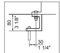
DETAIL Top Hat Shoe for Subsurface Fixed
