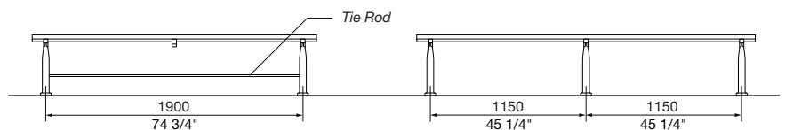
FRONT VIEW 2100L
