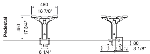
Surface Fixed
