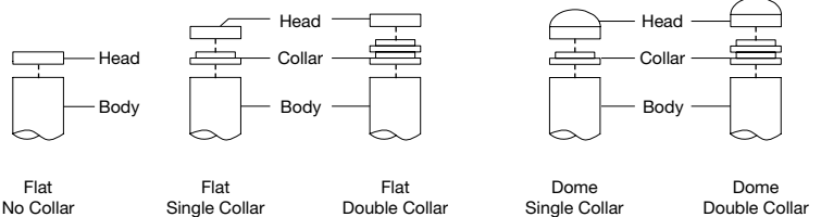
EXPLODED VIEW
