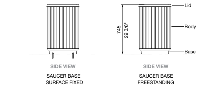
MOUNTING OPTIONS
