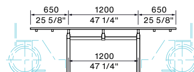
FRONT VIEW 2500L, DDA, Double End Access
