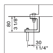
DETAIL Top Hat Shoe for Subsurface Fixed
