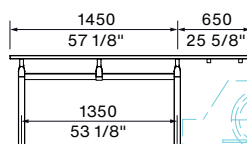
FRONT VIEW 2100L, DDA, Single End Access
