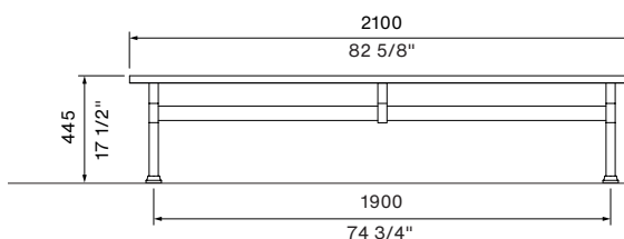
FRONT VIEW 2100mm
