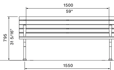
FRONT VIEW 1750mm
