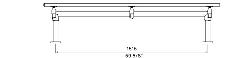
FRONT VIEW Surface Fixed
