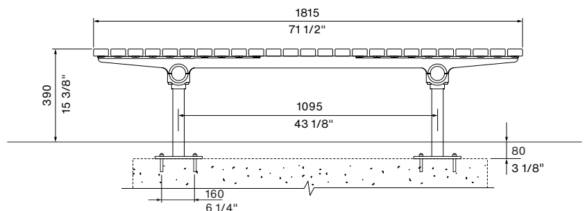
SIDE VIEW Subsurface Fixed
