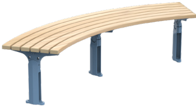
01 Mall Curved Slim Bench CMM8-C Pillar leg, aluminium Curly Birch battens, and Wedgewood frames. 440W x 445H x 1750L | 17 5/16" W x 17 1/2" H x 68 7/8" L
