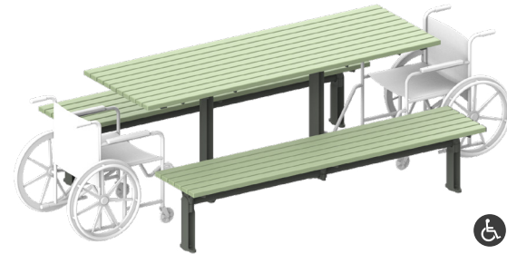
Mall DDA Table CMM6-DDA with Mall Slim Bench Pillar leg, Pale Eucalypt battens and Woodland Grey frame. Wheelchair access from both ends. 1600W x 850H x 2100L | 63" W x 33 1/2" H x 82 5/8" L
