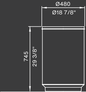
Simple Bin 80L (20-gal)
