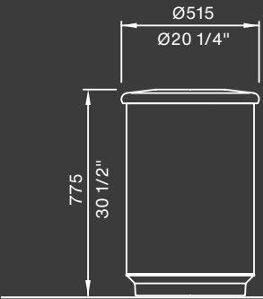
Plato Bin 80L (20-gal)
