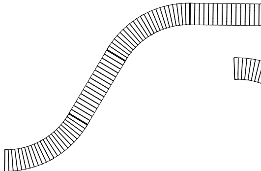
EXTENDED S-SHAPE QTY: 2 CURVED BENCHES + 2 BENCHES 3490 W x 5250 L (mm) 137 3/8" W x 206 3/4" L
