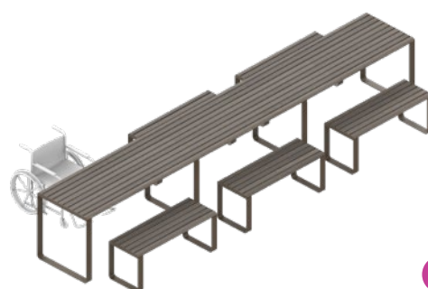
Linea Long Communal Table with Linea Bench Aluminium Beach Oak battens and Textura Dark Bronze frames. 750W x 840H x 5000L | 29 1/2" W x 33 1/8" H x 196 7/8" L
