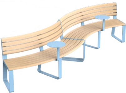
Linea Curved Seat with Table Accessory convex and concave Aluminium Curly Birch battens and Horizon Blue frames, freestanding. 1010W x 790H x 3730L | 39 3/4" W x 31 1/8 H x 146 7/8" L
