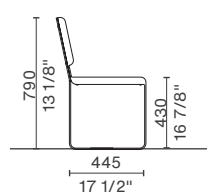
Seat with Square Leg To seamlessly align seats and benches when placed side-by-side.
