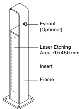
ISOMETRIC VIEW
