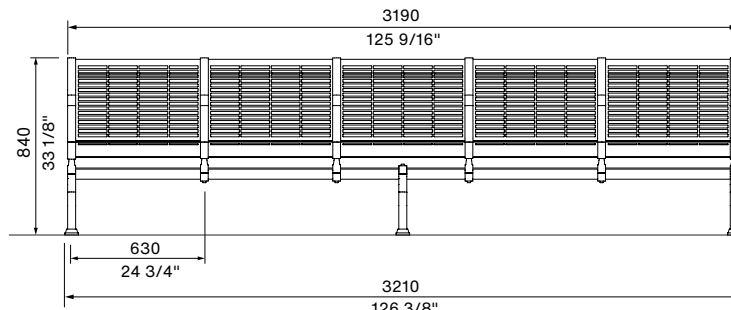
FRONT VIEW 5-SEATER
