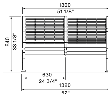
FRONT VIEW 2-SEATER
