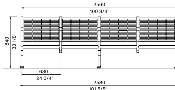
FRONT VIEW 4-SEATER
