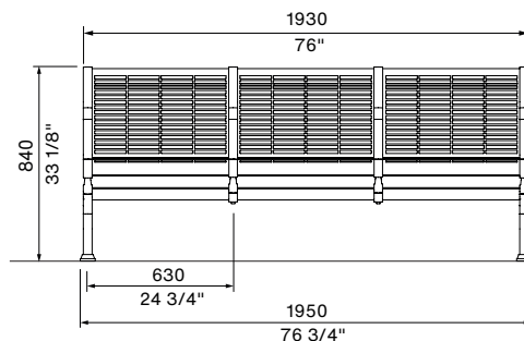
FRONT VIEW 3-SEATER
