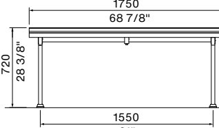
FRONT VIEW Standard
