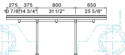
FRONT VIEW DDA Both End Access
