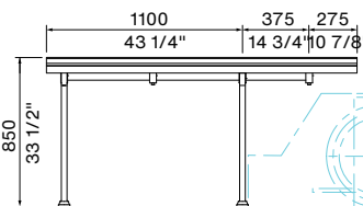
FRONT VIEW DDA Single End Access
