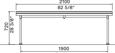
FRONT VIEW Standard
