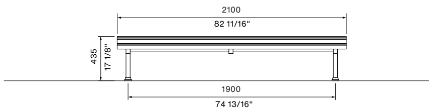
FRONT VIEW 2100mm
