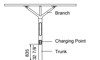
FRONT VIEW Powered
