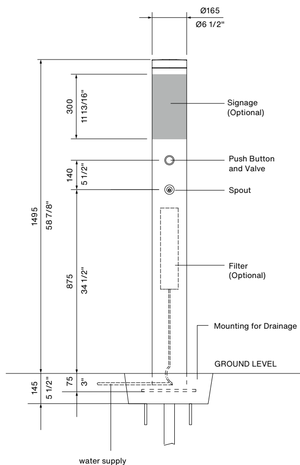
FRONT VIEW
