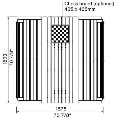
Setting 1: Aria Table and Seat (1800mm)
