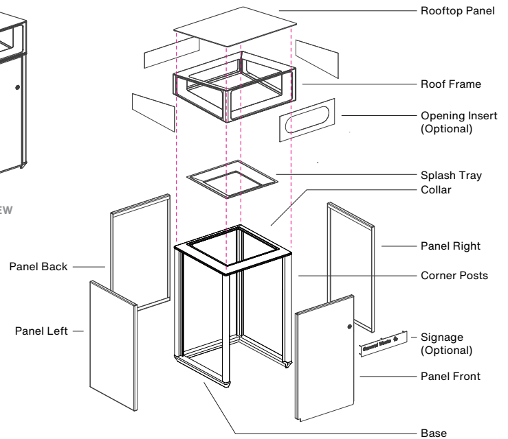
EXPLODED VIEW
