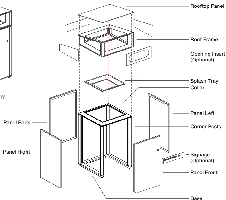
EXPLODED VIEW
