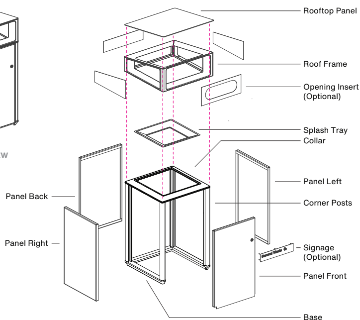
EXPLODED VIEW
