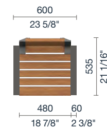
1S / 1SR (reversed) One Person Seat
