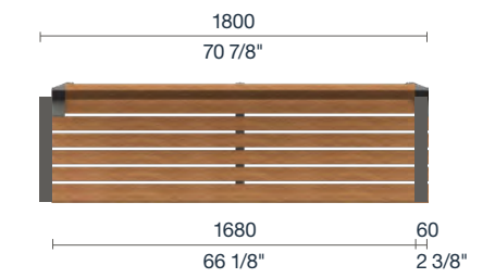
3S / 3SR (reversed) Three Person Seat
