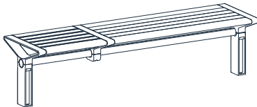
Aria Bench with Connect 180 2B-C180 480W x 1740L x 440H | 18 7/8" W x 68 1/2" L x 17 5/16" H
