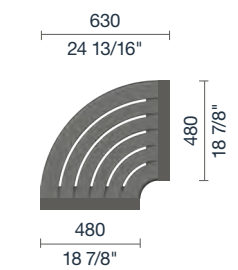
C90 Connect with 90° Panel
