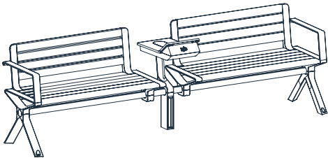
Aria Seats with PowerMe Table 2S-PM-2S 535W x 2700L x 790H | 21 1/16" W x 106 5/16" L x 31 1/8" H
