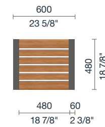
C180 Connect with 180° Panel
