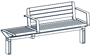
Aria Seat with Connect 180 2S-C180 535W x 1740L x 790H | 21 1/16" W x 68 1/2" L x 31 1/8" H
