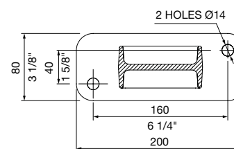
BASEPLATE DETAIL
