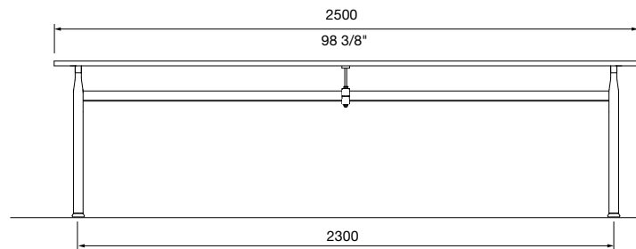
FRONT VIEW 2500 mm
