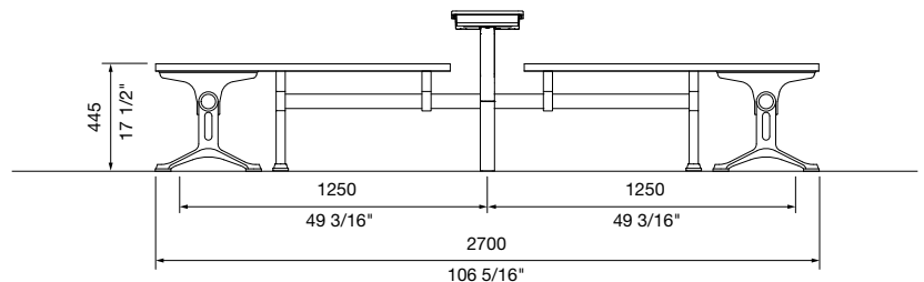
FRONT VIEW 2 PLUS 2 WITH POWERME TABLE
