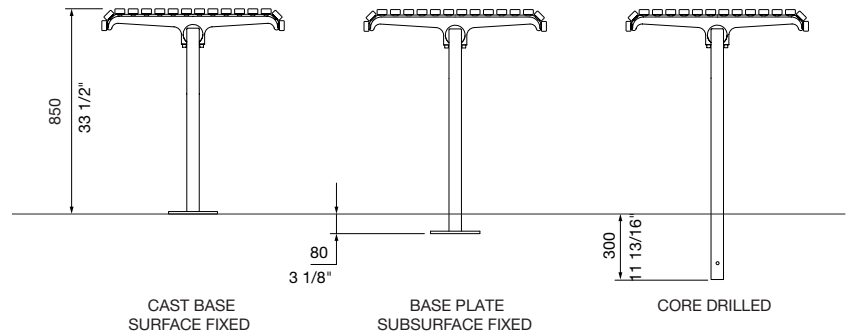
LEG AND MOUNTING OPTIONS
