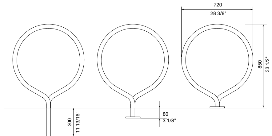
CORE DRILLED
