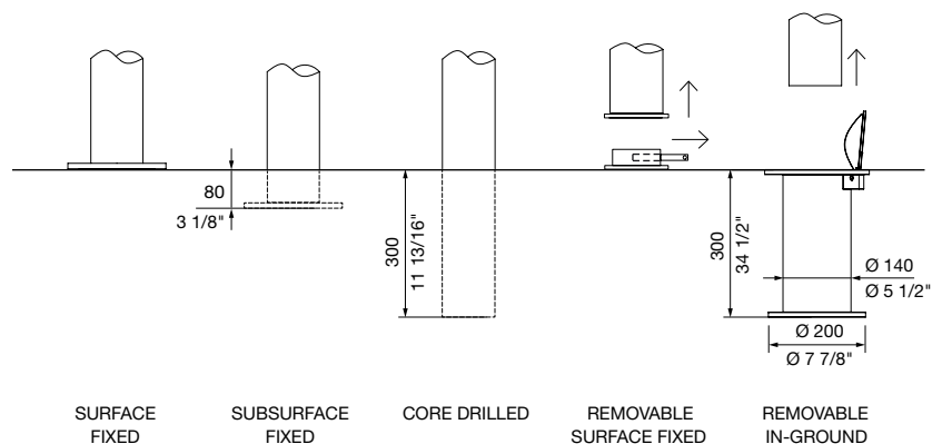
MOUNTING OPTIONS
