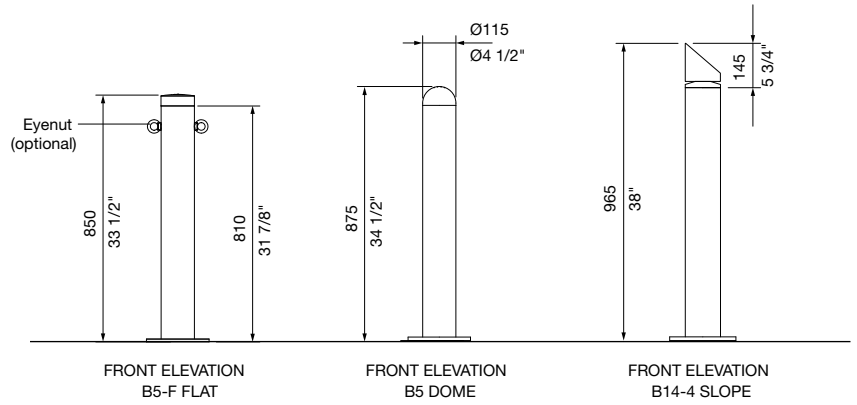
HEAD OPTIONS
