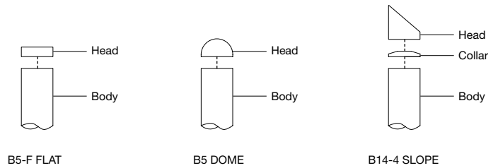
EXPLODED VIEW
