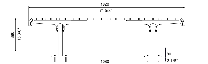
SIDE VIEW SUBSURFACE FIXED
