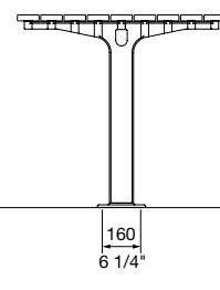
SIDE VIEW SURFACE FIXED
