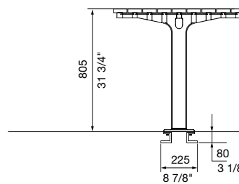
SIDE VIEW SUBSURFACE FIXED
