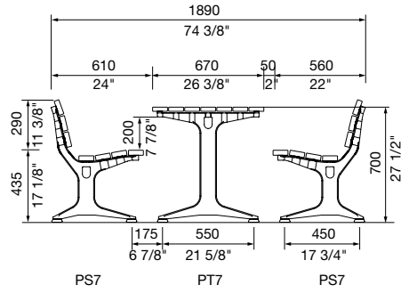
PS7 PT7 PS7 SIDE VIEW
