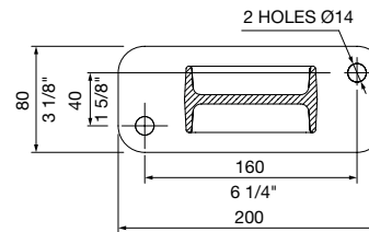
BASEPLATE DETAIL
