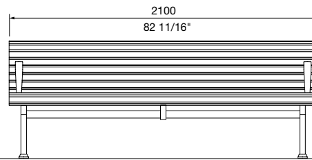
FRONT VIEW 2100mm
