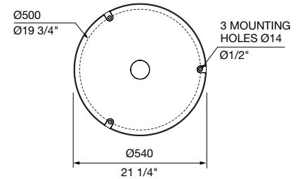
PLAN VIEW Cast Base
