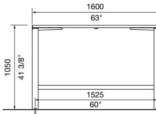
FRONT VIEW SURFACE FIXED
