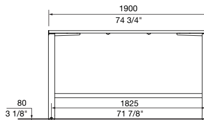
FRONT VIEW SUBSURFACE FIXED
