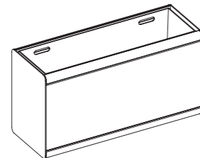
Long Rectangular M 1200L x 445W x 650H 47 1/4" L x 17 1/2" W x 25 5/8" H Soil volume ≈146 L
