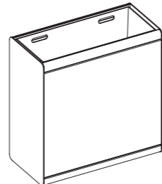
Rectangular L 900L x 445W x 940H 35 3/8" L x 17 1/2" W x 37" H Soil volume ≈106.5 L
