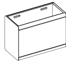
Rectangular M 900L x 445W x 650H 35 3/8" L x 17 1/2" W x 25 5/8" H Soil volume ≈106.5 L
