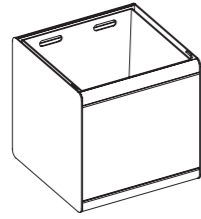
Square M 640L x 640W x 650H 25 1/4" L x 25 1/4" W x 25 5/8" H Soil volume ≈118 L
