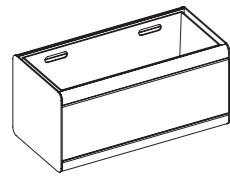
Rectangular S 900L x 445W x 435H 35 3/8" L x 17 1/2" W x 17 1/8" H Soil volume ≈61 L
