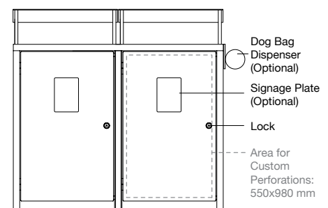
FRONT VIEW Angled Roof
