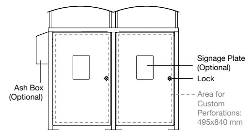
FRONT VIEW Curved Roof
