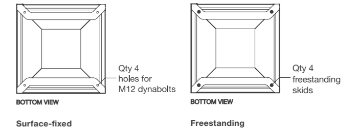
Surface-fixed
