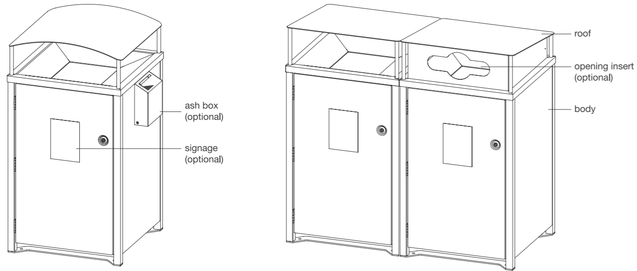
Frame Bin Enclosure with panels Curved roof, single unit. 120L WBE-F120-PAN | 640W x 640D x 1210H (mm) 240L WBE-F240-PAN | 700W x 810D x 1350H (mm)
