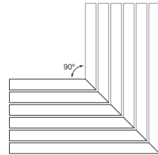
Mitred Corner 90° (Hardwood only)
