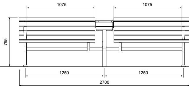
FRONT VIEW 2 PLUS 2 WITH POWERME TABLE
