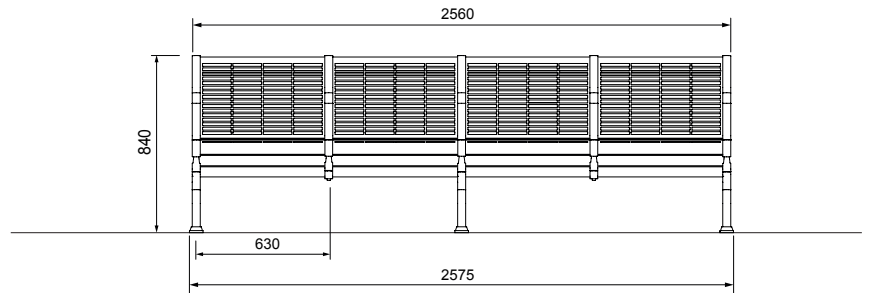
FRONT VIEW 4-SEATER
