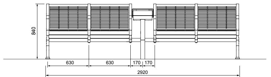
FRONT VIEW 2 PLUS 2 WITH POWEME TABLE
