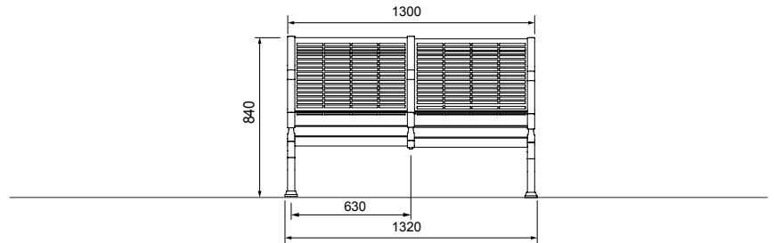
FRONT VIEW 2-SEATER
