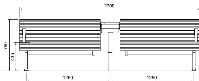
FRONT VIEW 2 PLUS 2 WITH POWERME TABLE
