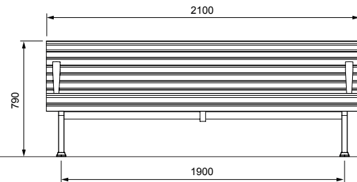
FRONT VIEW 2100mm
