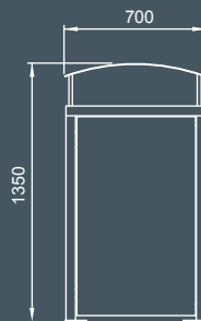
Frame Bin Enclosure 240L WBE-F240 700W x 810D x 1350H (mm)
