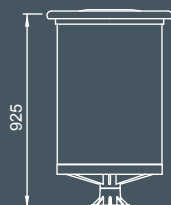
Rim Bin 80L LB2 with Hoop base Ø570 x 925H (mm)
