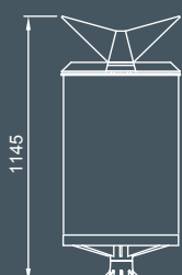
Monsoon Bin 80L LB8 with Hoop base Ø515 x 1145H (mm)
