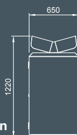
Monsoon Bin Enclosure 120L WBE-M120 650W x 650D x 1220H (mm)
