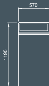
Escola Bin Enclosure 120L WBE-E120 570W x 590D x 1195H (mm)
