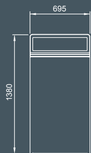
Escola Bin Enclosure 240L WBE-E240 695W x 760D x 1380H (mm)
