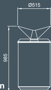
Monsoon Bin 80L LB8 with Saucer base Ø515 x 985H (mm)
