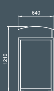
Frame Bin Enclosure 120L WBE-F120 640W x 640D x 1210H (mm)
