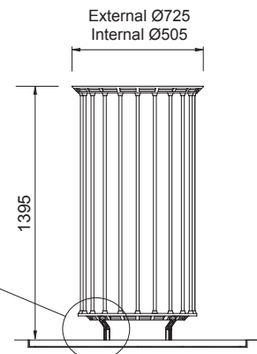
ELEVATION INTEGRATE SYSTEM
