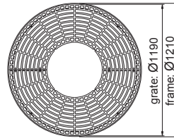
Round Treegrate GR1
