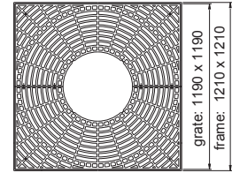
Square Treegrate GR2
