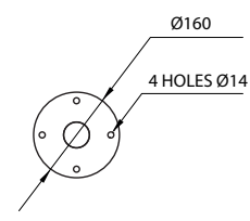
PLAN VIEW OF BASE PLATE
