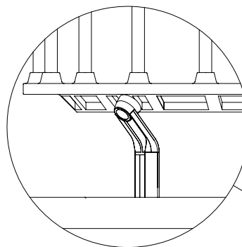
DETAIL VIEW TREEGUARD FOOT
