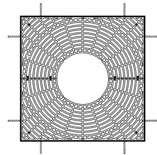
SQUARE GRATE 1210 x 1210 | 47 5/8" x 47 5/8"
