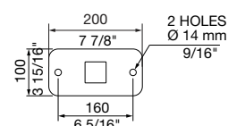
BASEPLATE DETAIL
